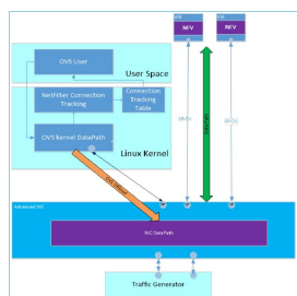
Connection Tracking (CT) - Open Virtual
